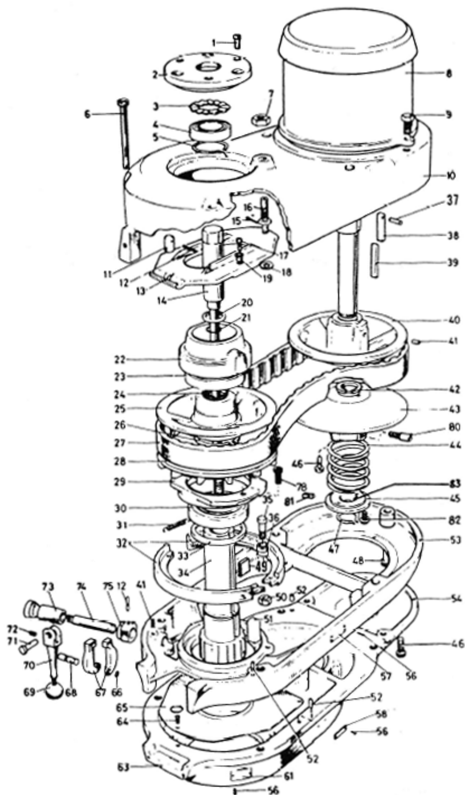
Figure 4.2 - 2J-Head Assembly
